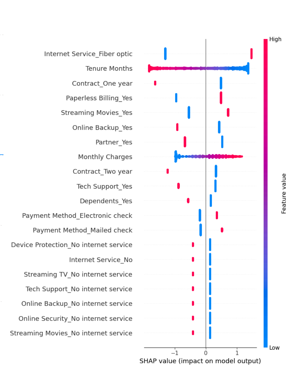
SHAP values of the model
